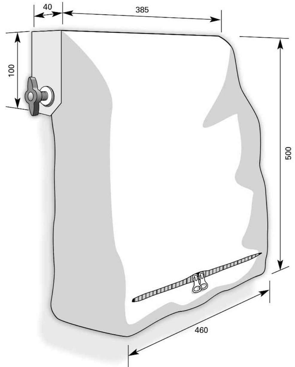
Dimensions shown in millimetres
